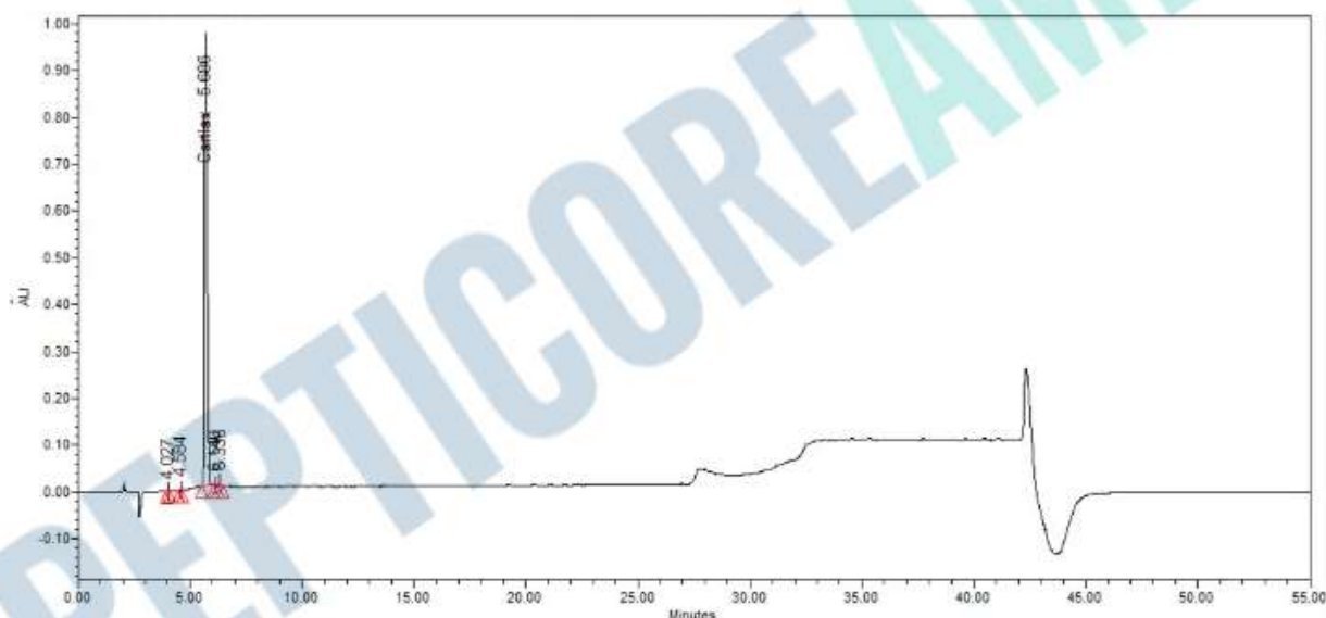
Figure 1: HPLC Chromatogram of Cartalax, PC-CX25-1512U (Auto Scale)
