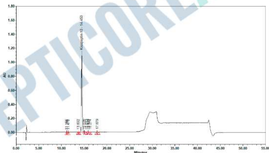
Figure 1: HPLC Chromatogram of Kisspeptin-10, PC-KIS10-1511U (Auto Scale)
