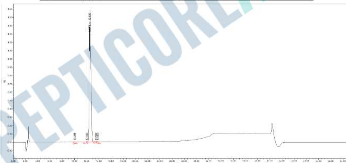
Figure 1: HPLC Chromatogram of MOTS-c, PC-MOTC-3010U (Auto Scale)
