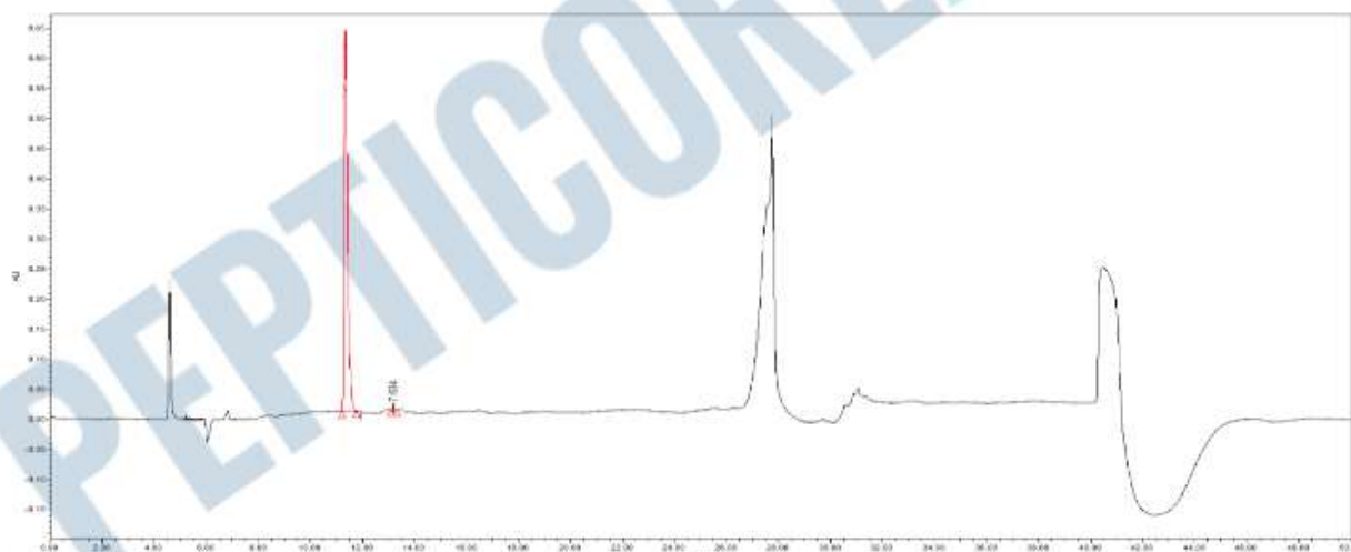
Figure 1: HPLC Chromatogram of SNAP-8, PC-SNAP10-1311U (Auto Scale)
