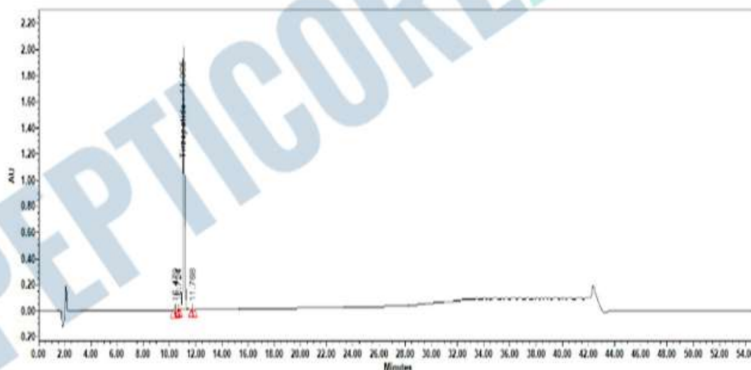
Figure 1: HPLC Chromatogram of Tirzepatide, PC-TIZ6-2507T (Auto Scale)
